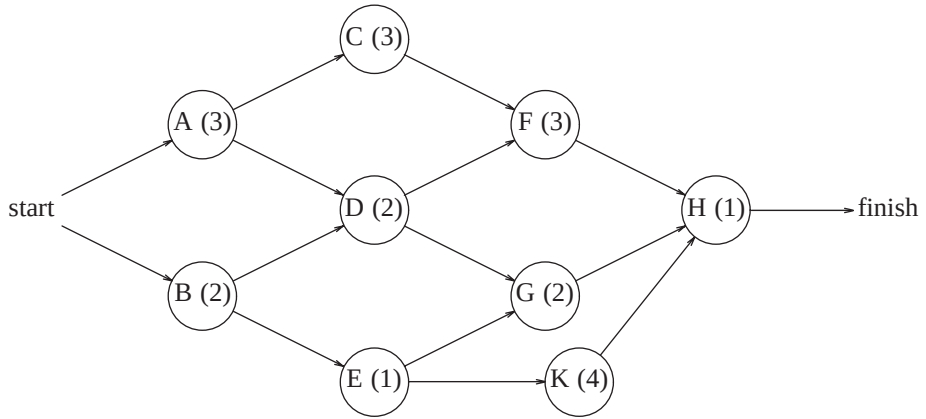
Figure 9.33 Activity-node graph
